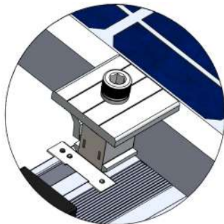
DETALLE B UNIVERSAL CLAMP (MODO - END)
