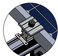
DETALLE A UNIVERSAL CLAMP (MODO - END)
