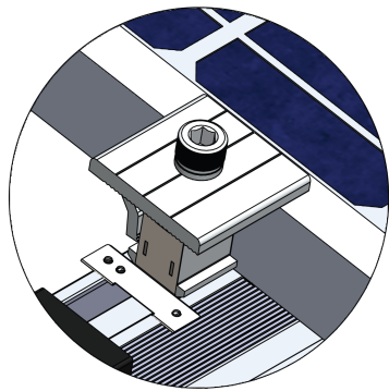
DETALLE B UNIVERSAL CLAMP (MODO - END)
