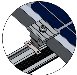
DETALLE C CLAMP UNIVERSAL (MODO - END)
