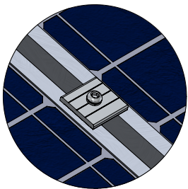
DETALLE D CLAMP UNIVERSAL (MODO - MID)
