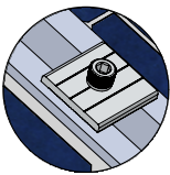
DETALLE A UNIVERSAL CLAMP (MODO - MID)
