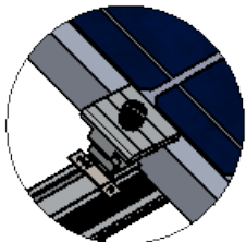
DETALLE C UNIVERSAL CLAMP (MODO-END)
