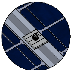
DETALLE B UNIVERSAL CLAMP (MODO - MID)
