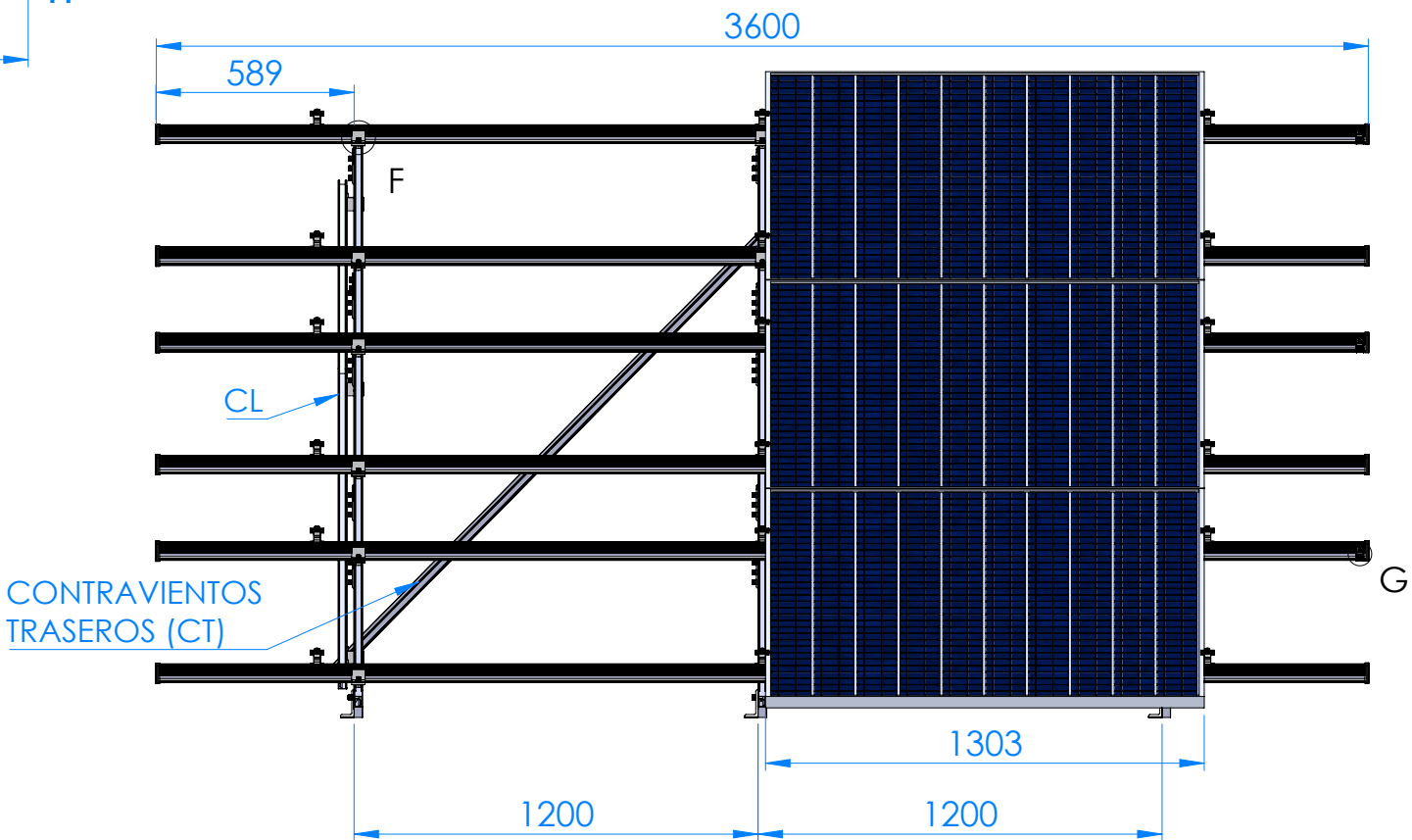
VISTA FRONTAL
