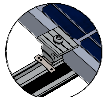
DETALLE C UNIVERSAL CLAMP (MODO - END)
