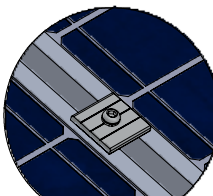
DETALLE D UNIVERSAL CLAMP (MODO - MID)
