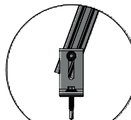
DETALLE G L-FOOT SUPPORT
