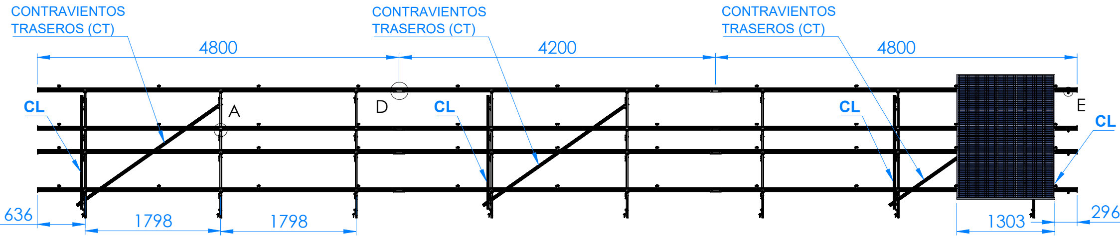
VISTA FRONTAL
