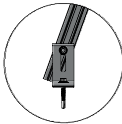
DETALLE G L-FOOT SUPPORT
