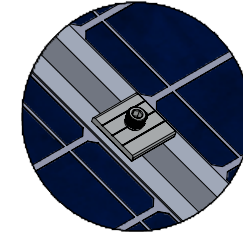
DETALLE B UNIVERSAL CLAMP (MODO-MID)
