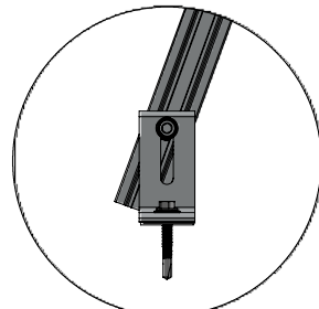
DETALLE G L-FOOT SUPPORT
