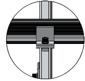
DETALLE A CLIP CLIMBER
