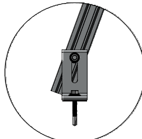
DETALLE G L-FOOT SUPPORT
