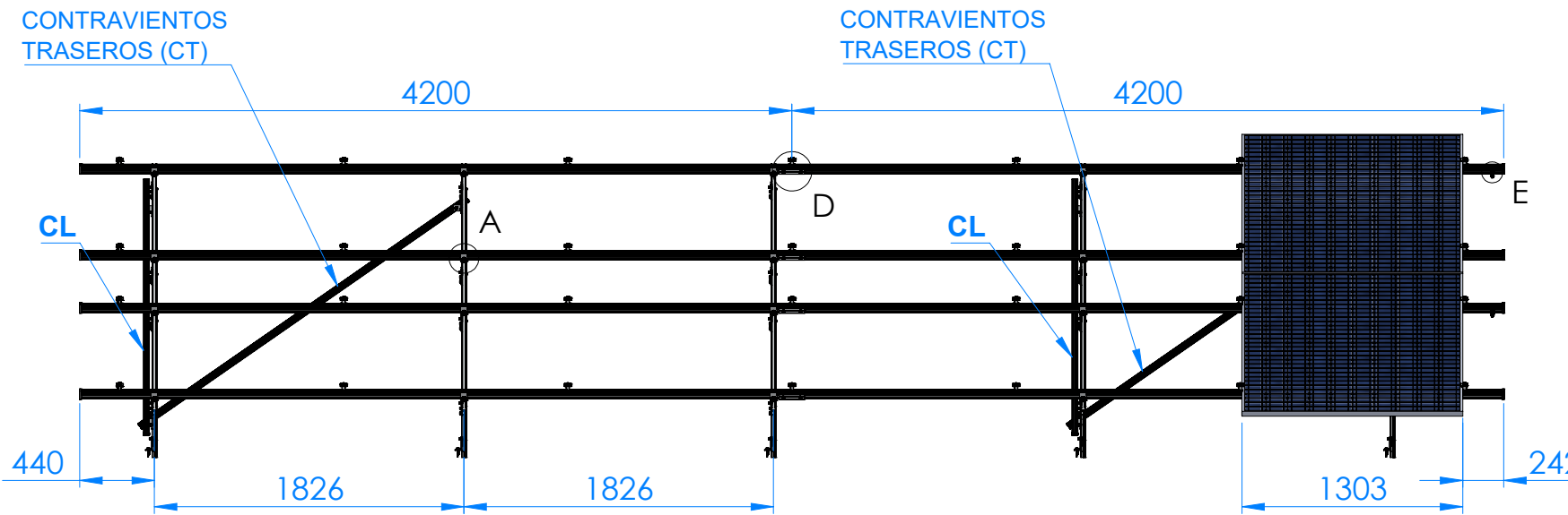
VISTA FRONTAL
